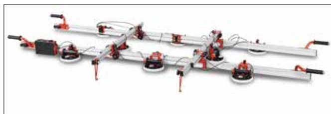
Power-Vacuum kit mounted on EASY-MOVE mini with crossbars (Art. 432HAKITR + Art. 432EM04TA).
