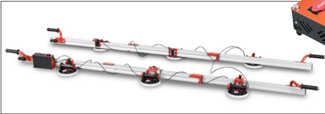
Power-Vacuum kit mounted on EASY-MOVE MkIV without crossbars (Art 432HAKITR + Art. 432EMO4CA).
