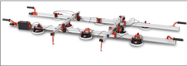
Power-Vacuum kit mounted on EASY-MOVE MkIV with crossbars (Art 432HAKITR + Art. 432EMO4TA).
